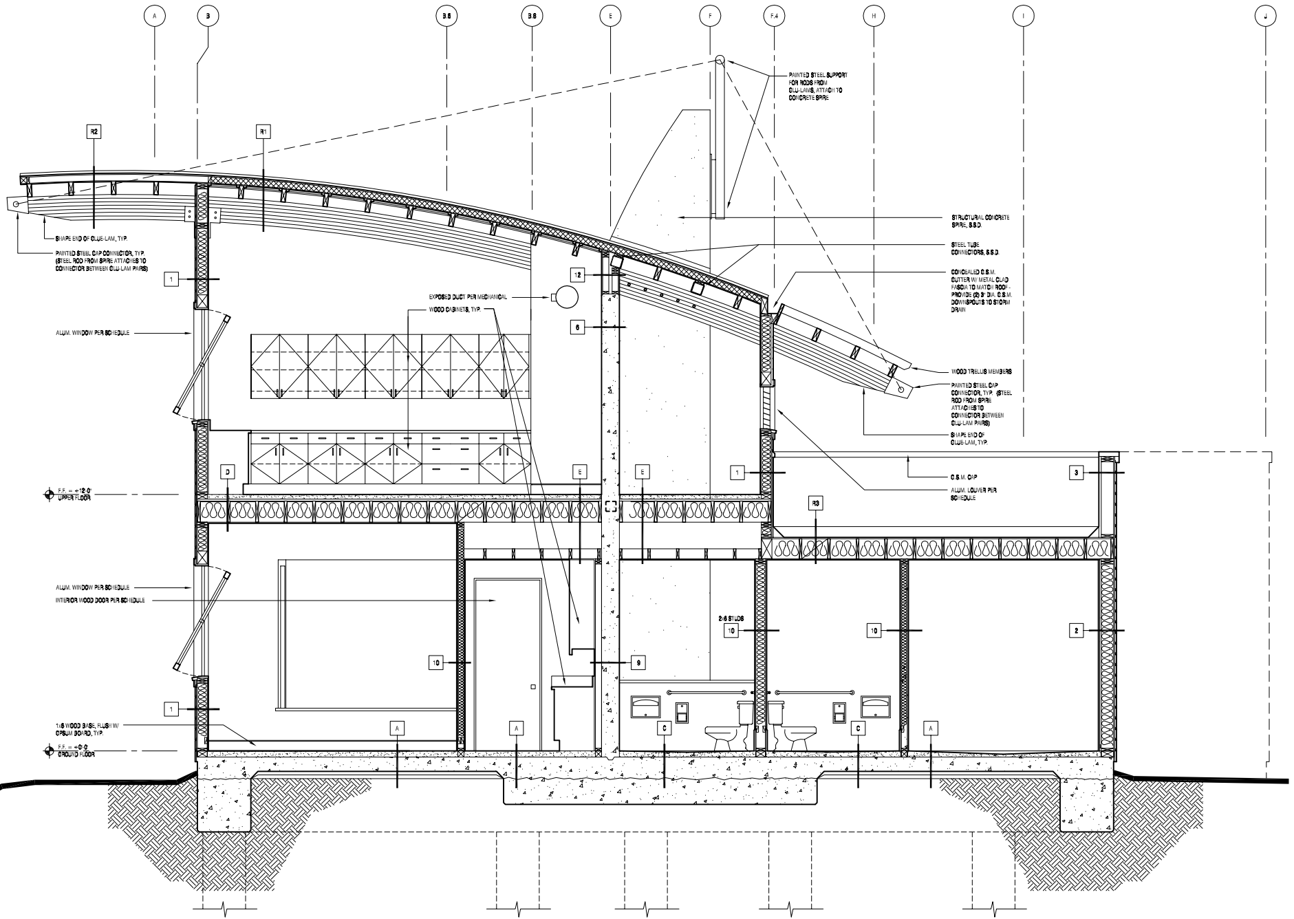
BUILDING SECTION 0 1' 2' 3' 4' 5'
